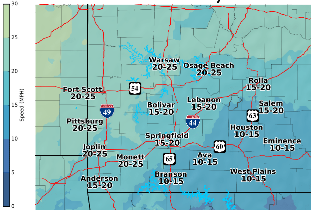
Maximum Wind Gusts – Tuesday
